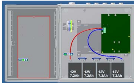
Fig. 1: Skitse over central 230V/48V 15A-1-1
