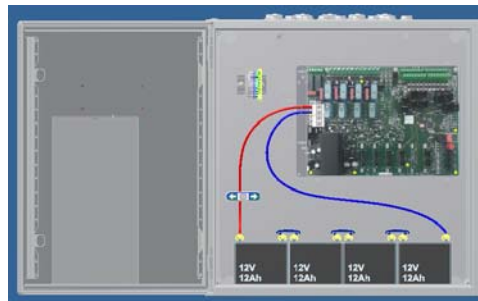
Fig. 2: Skitse over central 230V/48V 30A-2-1
